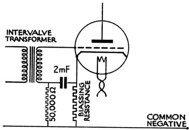
Automatic Bias for Indirectly-heated L.F. Amplifier.
