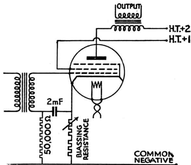
Automatic Bias for Indirectly-heated Triode or Pentode Output Valve.
