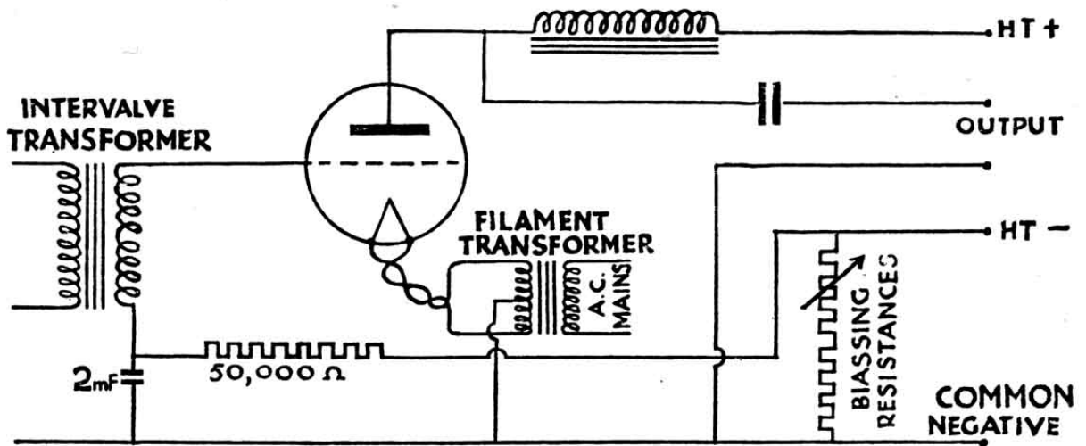
Automatic Bias for Directly-heated Triode or Pentode Output Valve.
